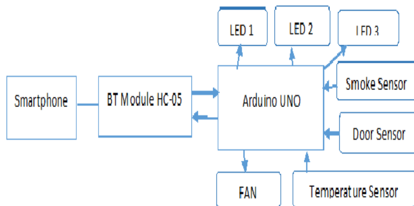
Fig 3. Block diagram of smart automation system using Bluetooth
