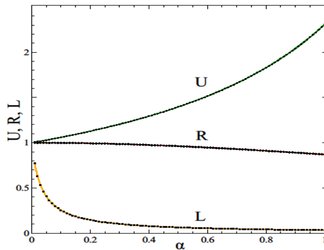
FIG 3: Figure shows that, as the degree of non-Markovianity \alpha is increased, the speed limit for correlated Markov noise increases for upper bound and for lower bound the speed limit decreases.
